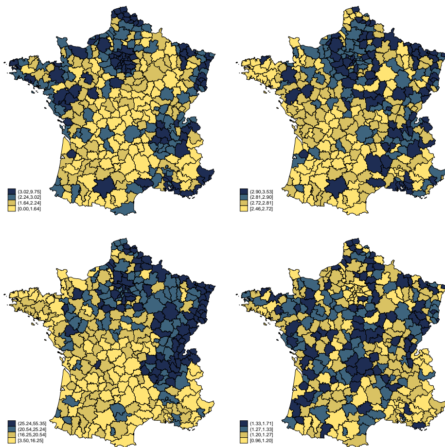
Figure 3: Spatial distribution of employment density (log, top left); TFP ( \omega , top right); export participation rate (in percentage, bottom left); markups ( \mu , bottom right), by employment area
